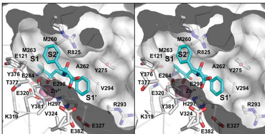
Figure 4 Stereoview of the surface diagram at the active site in the APN–PL250 complex. The S_1 , S_1' and S_2' subsites of E. coli APN are shown. The zinc ion and main chain are shown as a pink sphere and a C^\alpha trace, respectively. The residues constituting these subsites are represented using stick models. The PL250 stick model binding to the active site is in cyan. This diagram was drawn and rendered with the program PyMOL ( http://www.pymol.org/ ).
